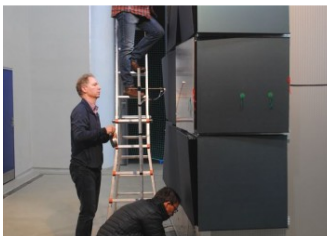
Prototype of the façade with Kingspan elements, solar modules, mounting system with brackets and rails, silicon joints, was built for tests © Solarlab
